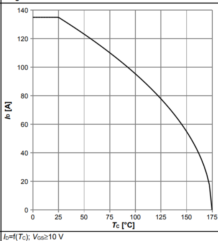
Diagram 2: Drain current
