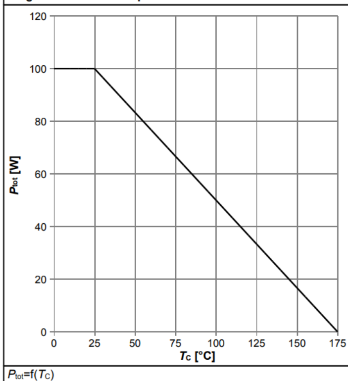
Diagram 1: Power dissipation
