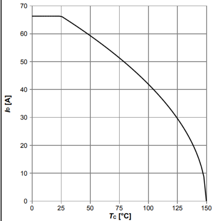
Diagram 2: Drain current
