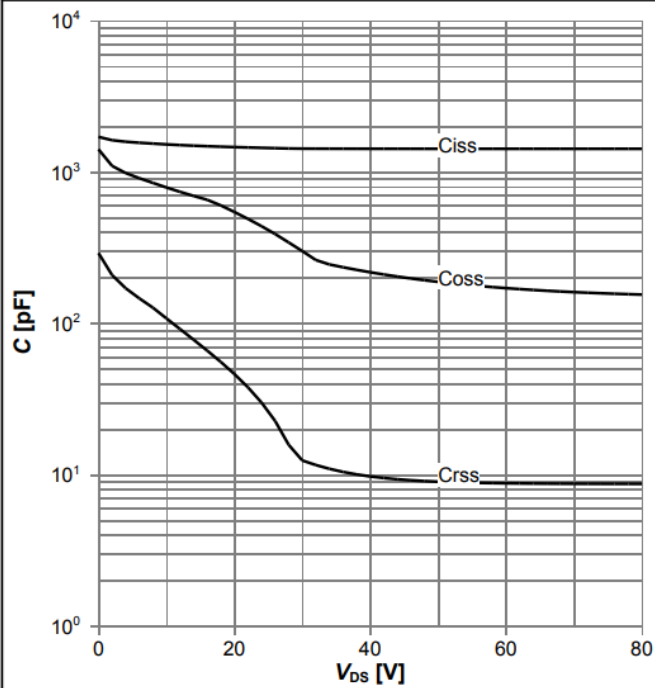
Diagram 11: Typ. capacitances
