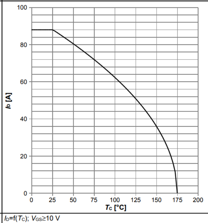
Diagram 2: Drain current
