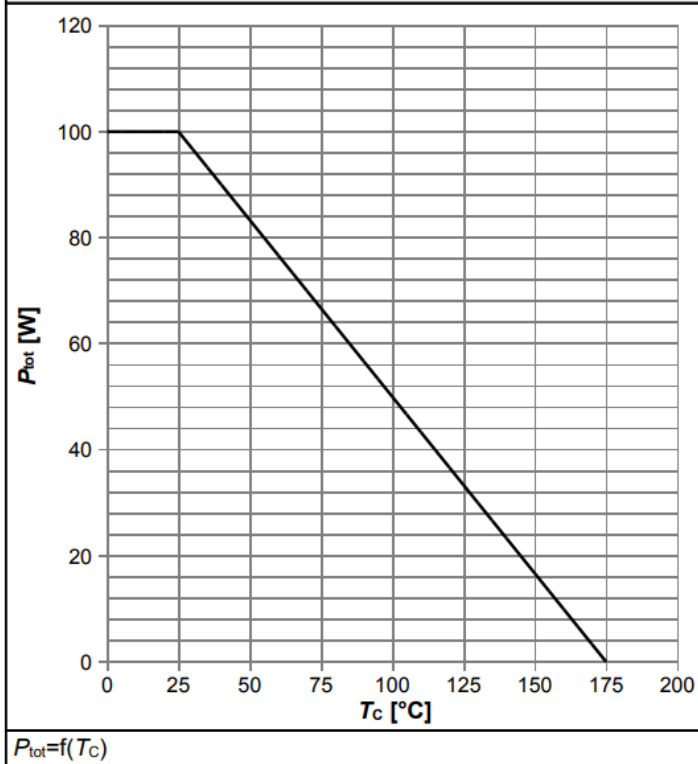
Diagram 1: Power dissipation
