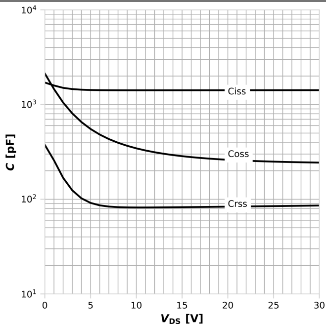
Diagram 11: Typ. capacitances
