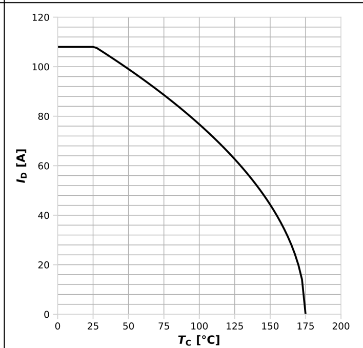
Diagram 2: Drain current
