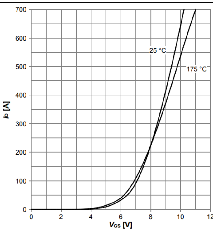
Diagram 8: Typ. transfer characteristics
