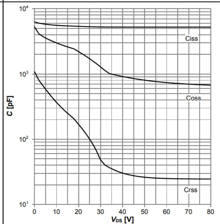
Diagram 12: Typ. capacitances
