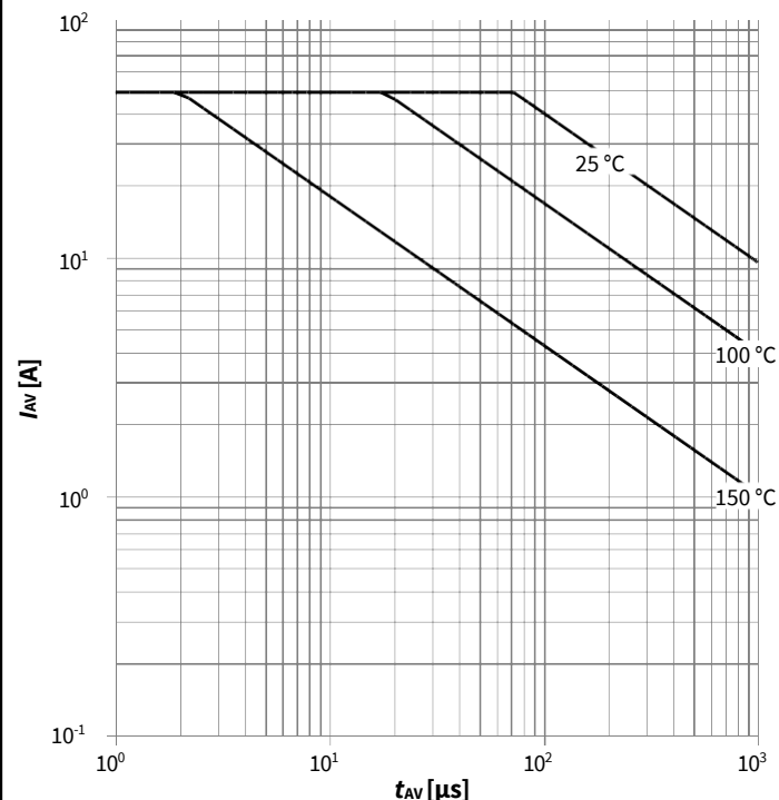
Diagram 13: Avalanche characteristics
