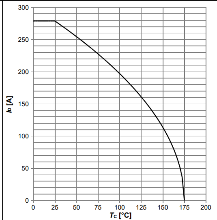
Diagram 2: Drain current
