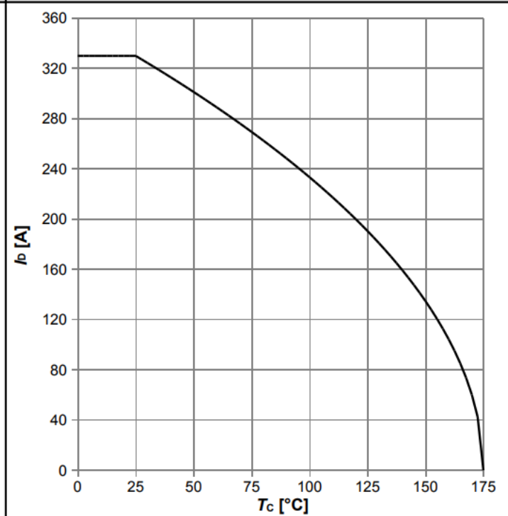
Diagram 2: Drain current
