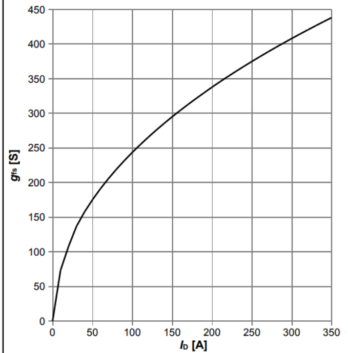
Diagram 8: Typ. transconductance
