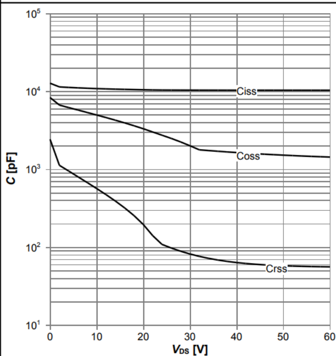
Diagram 11: Typ. capacitances
