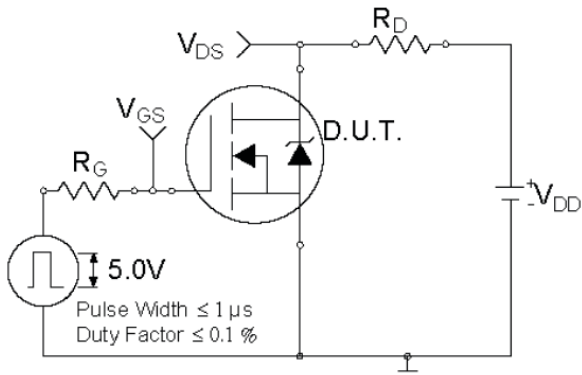
Fig 10b. Switching Time Test Circuit
