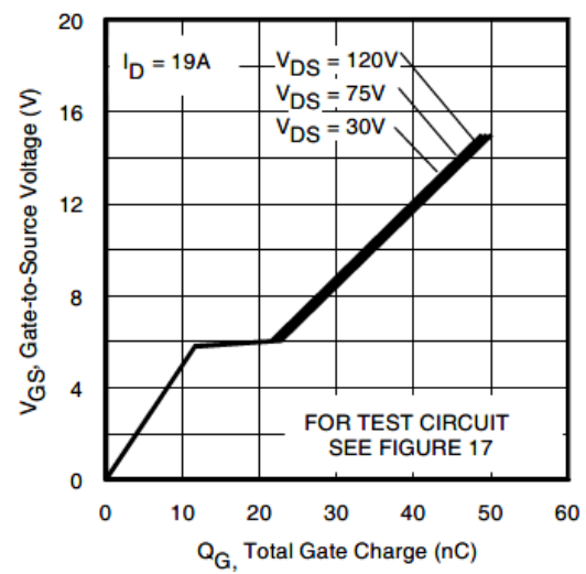
Figure 11 Typical Gate Charge Vs. Typical Gate-to-Source Voltage
