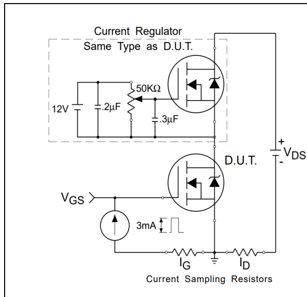
Figure 17 Gate Charge Test Circuit
