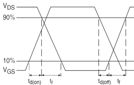
Figure 22 Switching Time Waveforms
