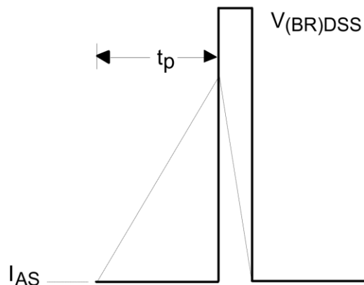
Figure 20 Unclamped Inductive Waveform
