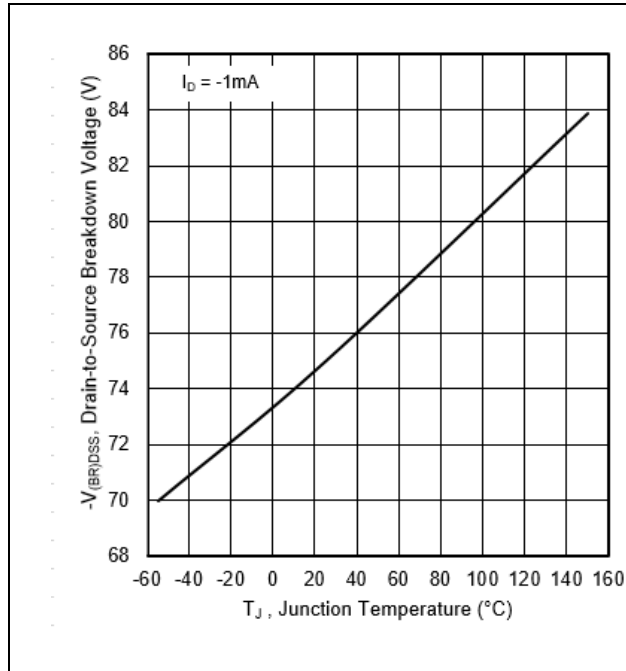
Figure 8 Typical Drain-to-Source Breakdown Voltage Vs. Temperature
