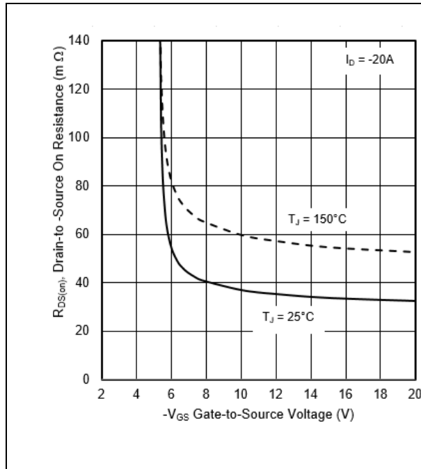
Figure 6 Typical On-Resistance Vs. Gate Voltage
