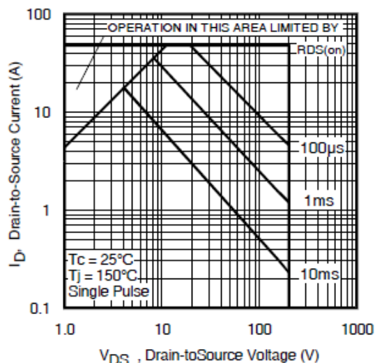
Fig 8. Maximum Safe Operating
