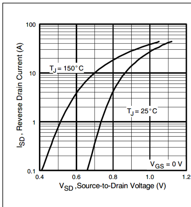
Figure 8 Typical Source-Drain Current Vs. Diode Forward Voltage
