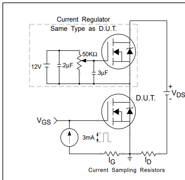
Figure 13 Gate Charge Test Circuit
