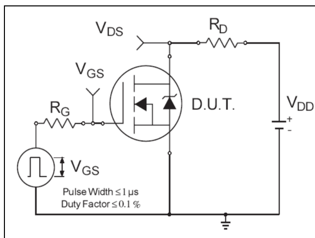
Figure 17 Switching Time Test Circuit
