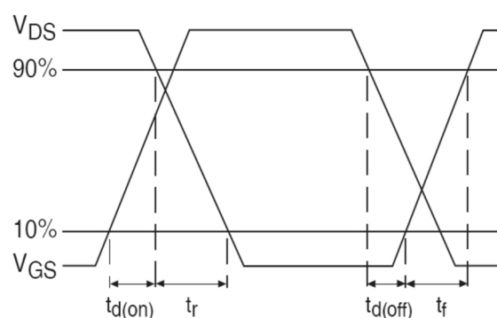
Figure 18 Switching Time Waveforms
