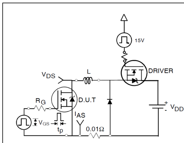
Figure 15 Unclamped Inductive Test Circuit
