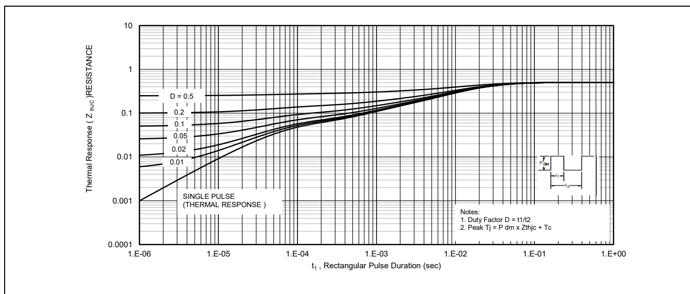
Figure 17 Maximum Effective Transient Thermal Impedance, Junction-to-Case
