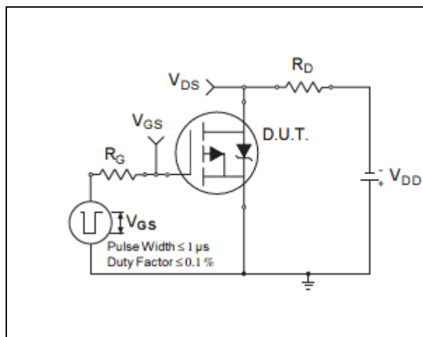
Figure 21 Switching Time Test Circuit
