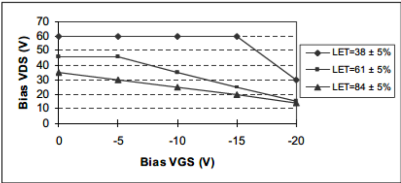
Figure 1 Typical Single Event Effect, Safe Operating Area
