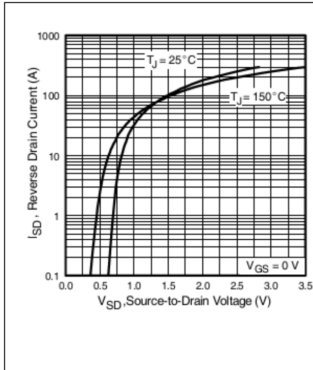
Figure 8 Typical Source-Drain Current Vs. Diode Forward Voltage
