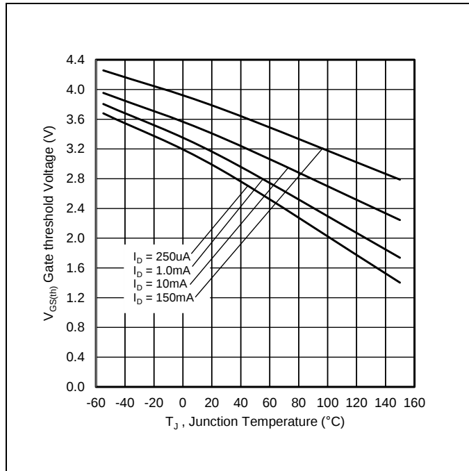
Figure 6 Typical Threshold Voltage Vs. Temperature
