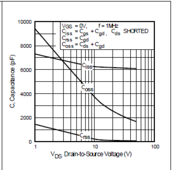
Figure 7 Typical Capacitance Vs. Drain-to-Source Voltage
