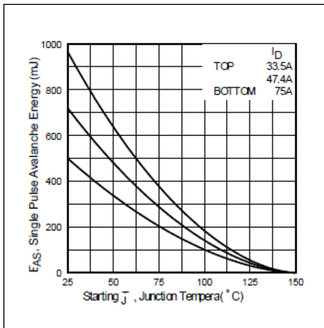
Figure 12 Maximum Avalanche Energy Vs. Junction Temperature
