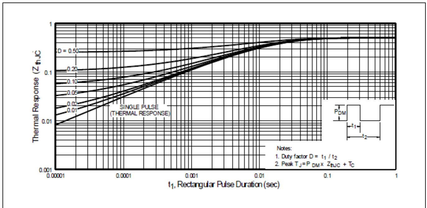
Figure 13 Maximum Effective Transient Thermal Impedance, Junction-to-Case
