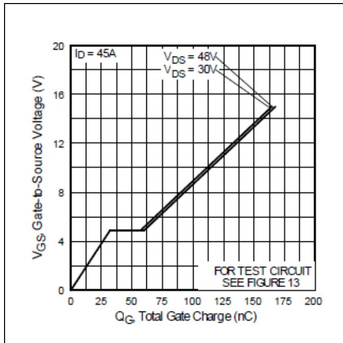
Figure 8 Typical Gate-to-Source Voltage Vs. Typical Gate Charge
