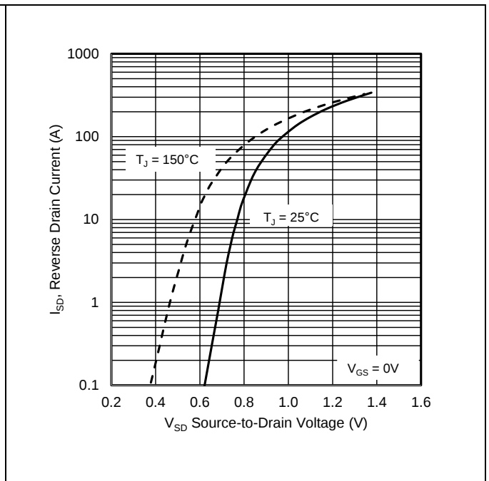
Figure 9 Typical Source-Drain Current Vs. Diode Forward Voltage
