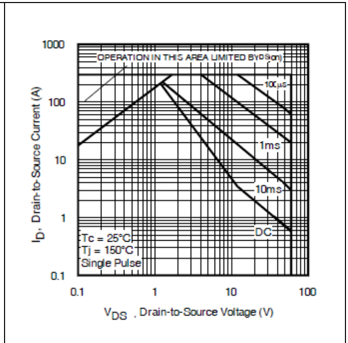
Figure 11 Maximum Safe Operating Area
