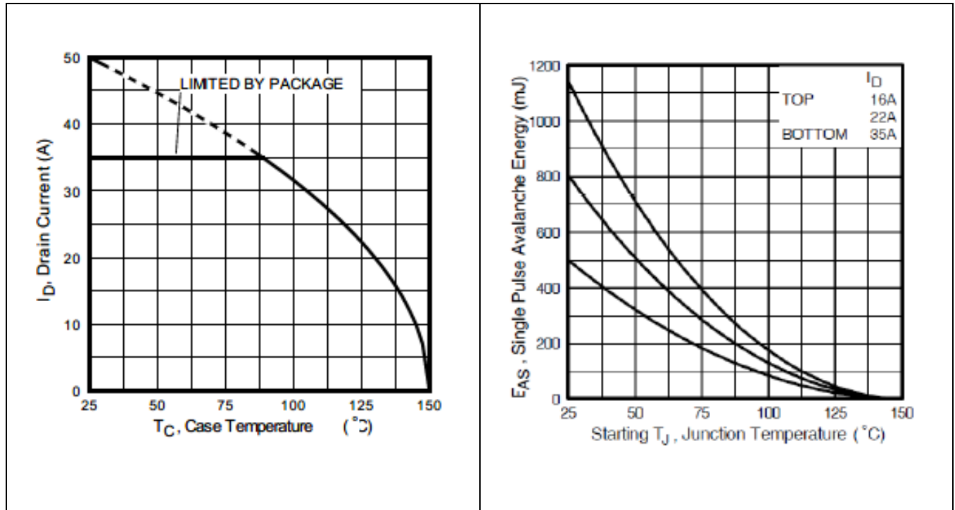
Figure 10 Maximum Drain Current Vs. Case Temperature
