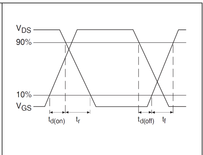
Figure 22 Switching Time Waveforms
