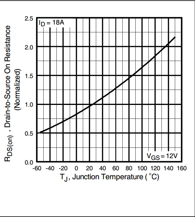
Figure 5 Normalized On-Resistance Vs. Temperature
