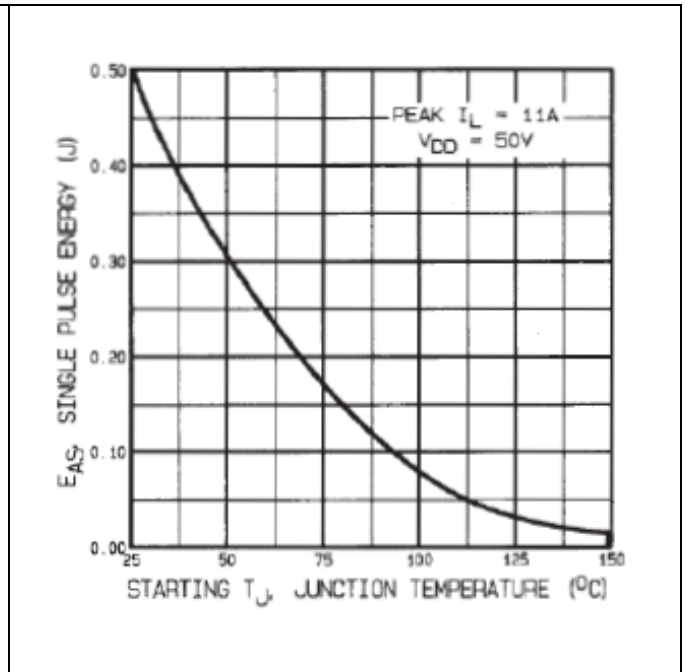
Figure 11 Maximum Avalanche Energy Vs. Junction Temperature
