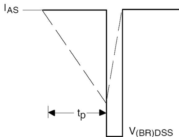
Fig 16b. Unclamped Inductive Wave-
