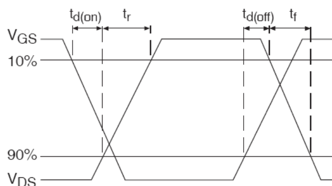
Fig 18b. Switching Time Waveforms
