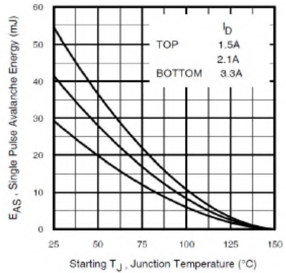
Figure 15 Maximum Avalanche Energy Vs. Junction Temperature
