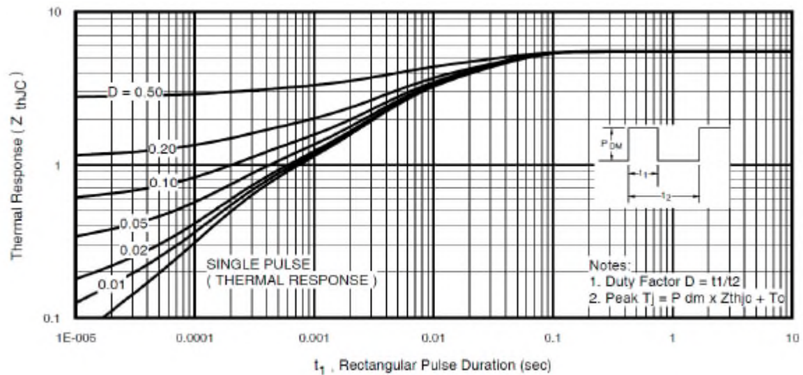
Figure 16 Maximum Effective Transient Thermal Impedance, Junction-to-Case
