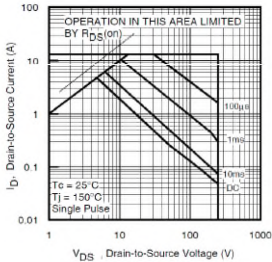
Figure 14 Maximum Safe Operating Area
