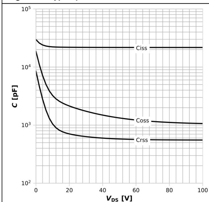
Diagram 11: Typ. capacitances
