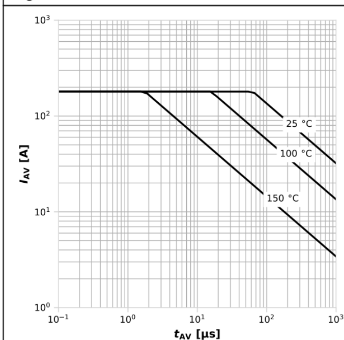
Diagram 13: Avalanche characteristics
