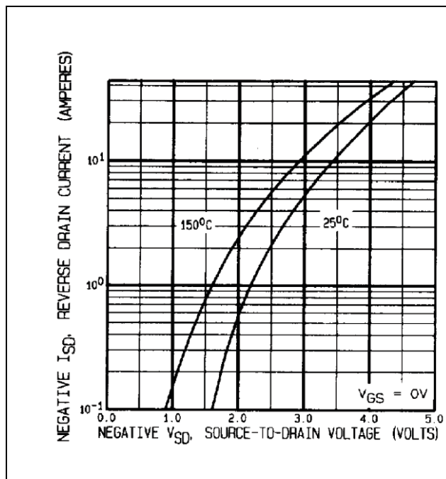
Figure 7 Typical Source-Drain Diode Forward Voltage
