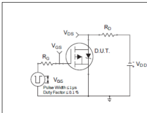
Figure 16 Switching Time Test Circuit
