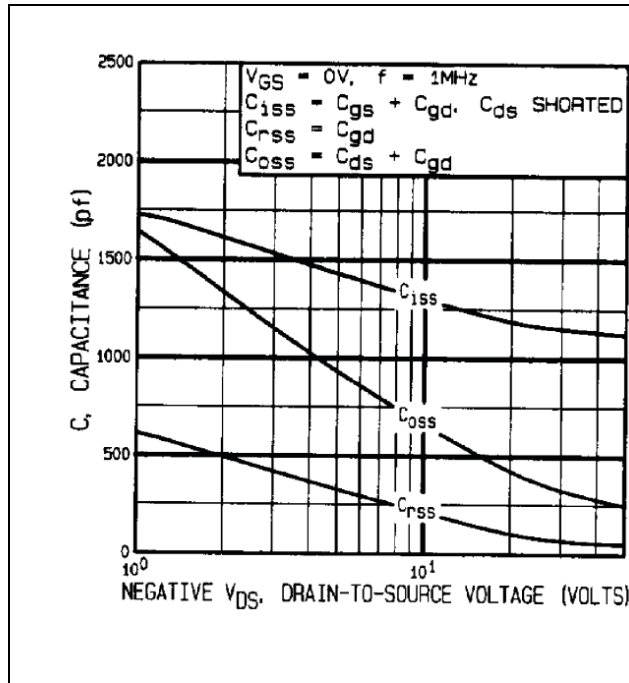
Figure 5 Typical Capacitance Vs. Drain-to-Source Voltage
