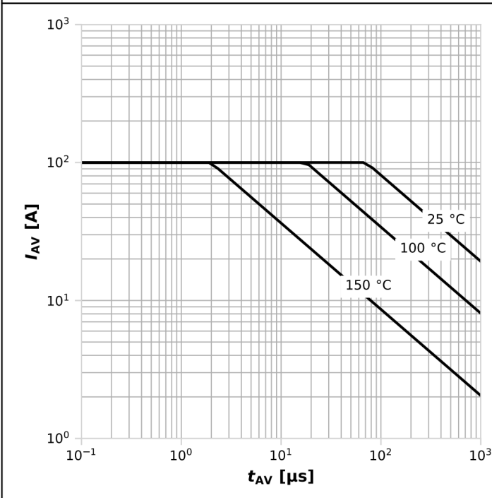
Diagram 13: Avalanche characteristics
