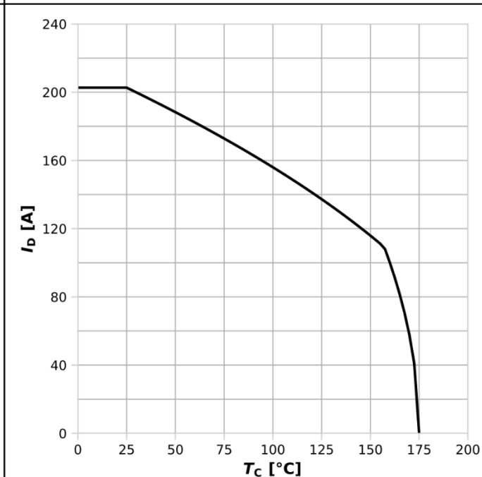
Diagram 2: Drain current
