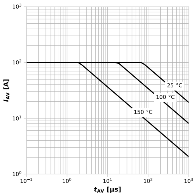
Diagram 13: Avalanche characteristics
