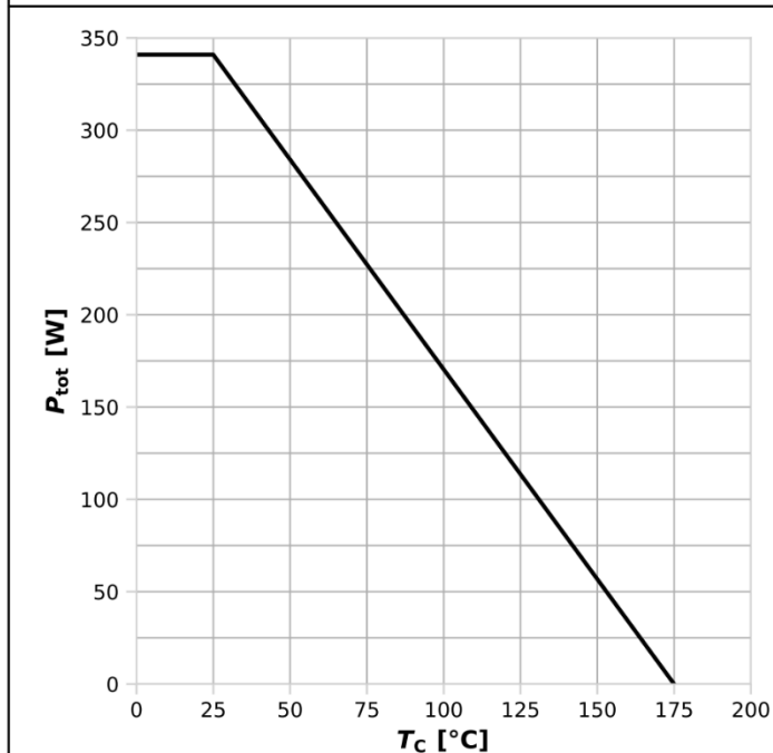
Diagram 1: Power dissipation
