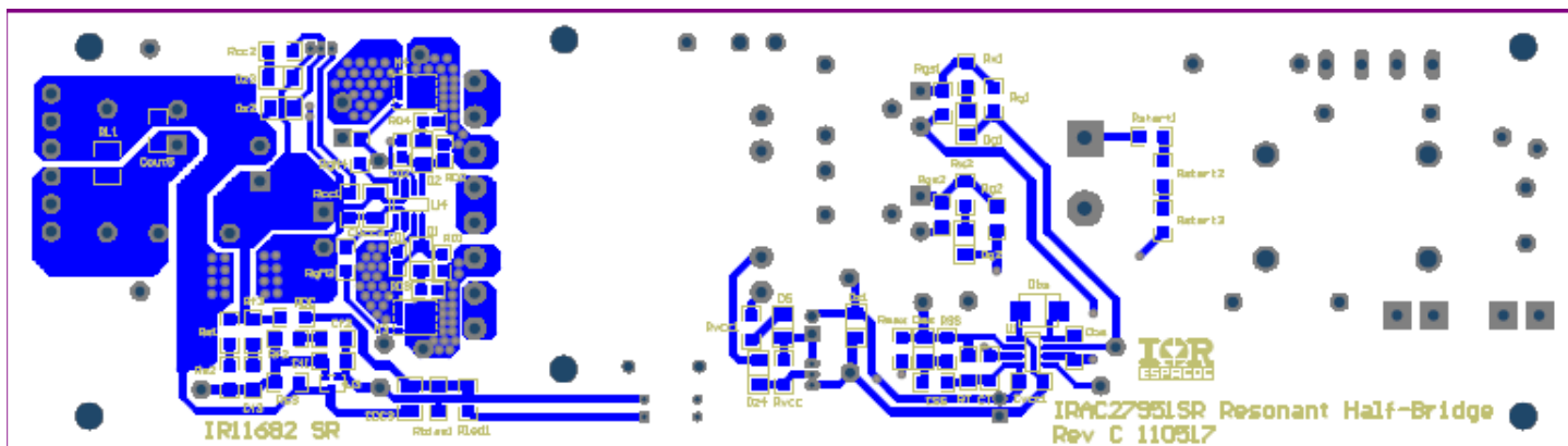
Figure 6 - Board Bottom Layer Copper
