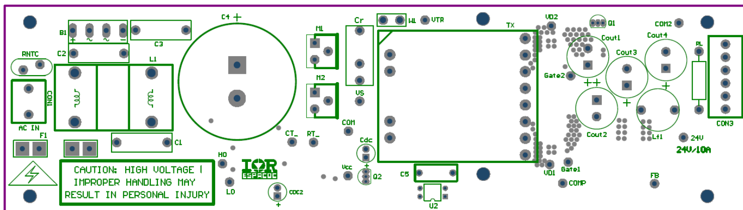
Figure 3 – Evaluation Board Top Side Component Placement
