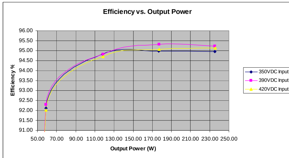
Figure 9 - Efficiency plot
