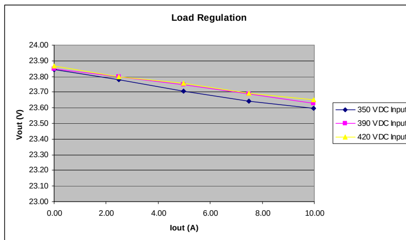
Figure 8 - Output voltage regulation plot
