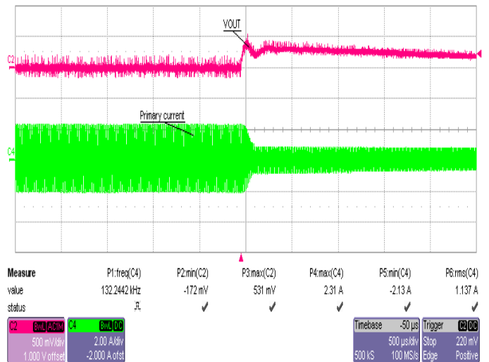
Full Load to No Load Step at 420Vdc
