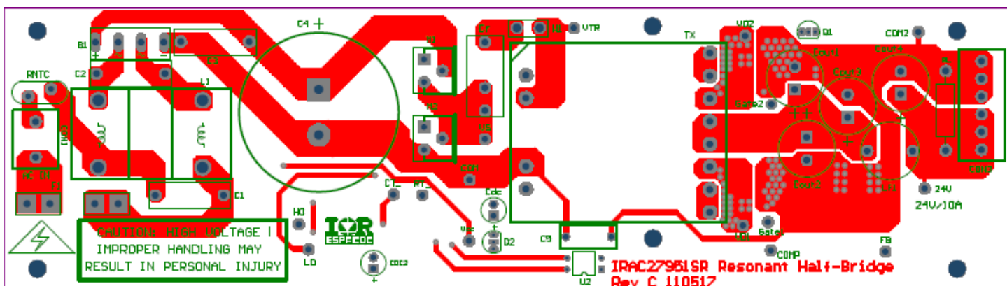
Figure 5 - Board Top Layer Copper
