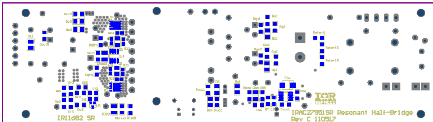
Figure 4 – Evaluation Board Bottom Side Component Placement
