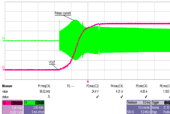
Full Load Start-up
