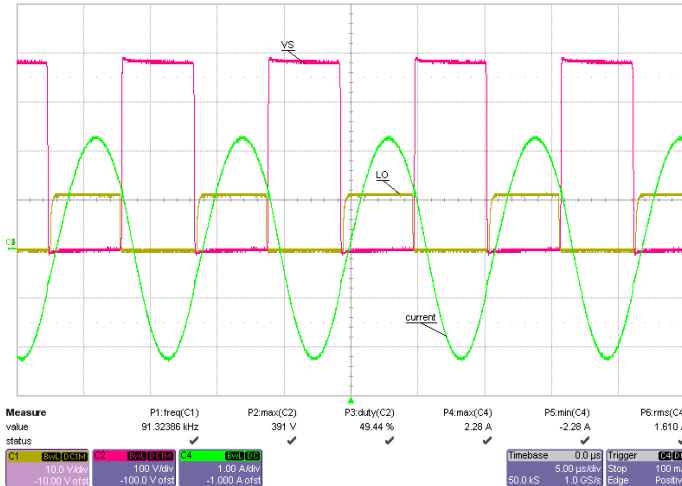
Full Load Operation
