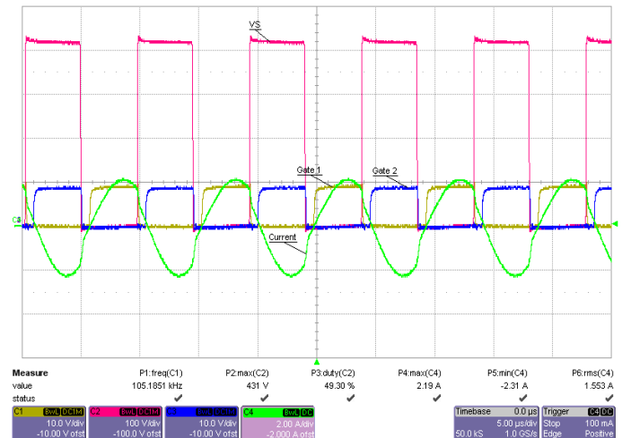
420Vdc, Full Load Operation
