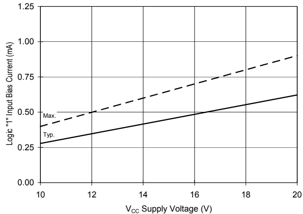
Fig 29b. Logic "1" Input Current Vs. Voltage
