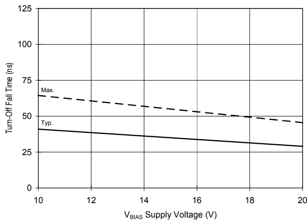
Fig 14b. Turn-Off Fall Time Vs. Voltage
