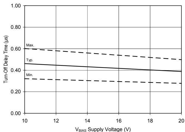
Fig 12b. Turn-Off Time Vs. Voltage
