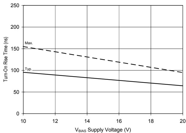
Fig 13b. Turn-On Rise Time Vs. Voltage
