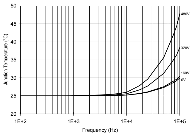
Fig 51. IR2130 T_J Vs. Frequency (IRF830) R_{GATE} = 20\Omega , V_{CC} = 15V
