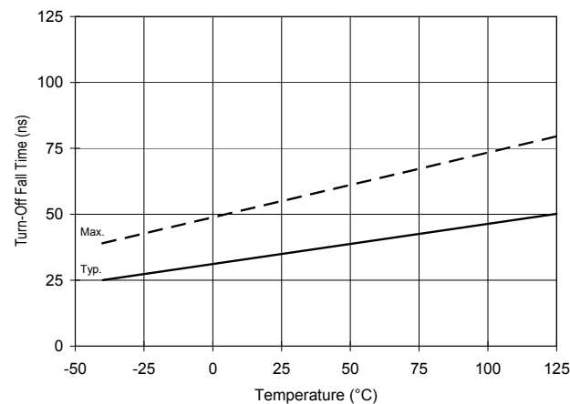
Fig 14a. Turn-Off Fall Time Vs. Temperature
