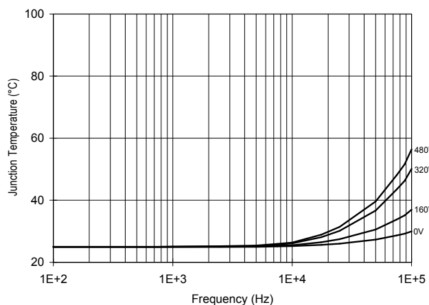
Fig 52. IR2130 T_J Vs. Frequency (IRF840) R_{GATE} = 15\Omega , V_{CC} = 15V
