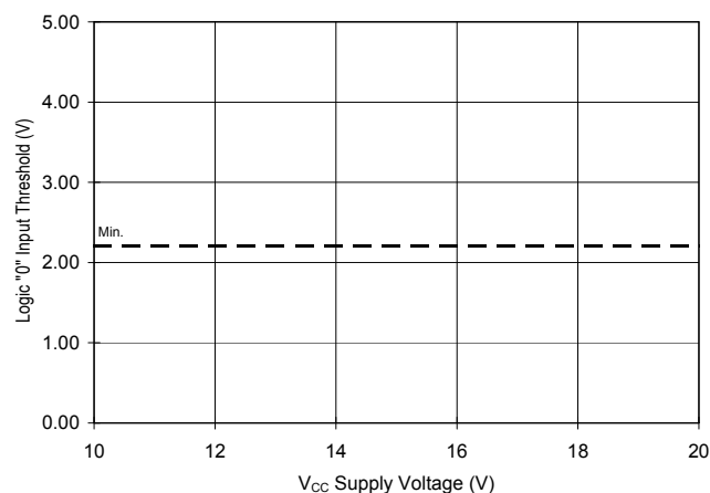
Fig 21b. Logic "0" Input Threshold Vs. Voltage
