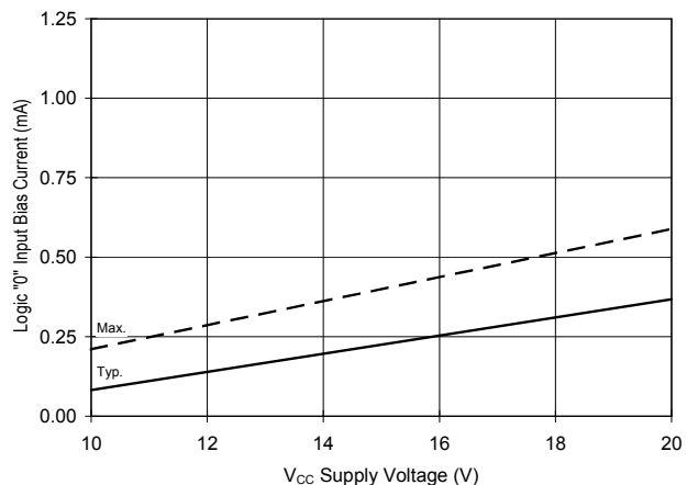
Fig 30b. Logic "0" Input Current Vs. Voltage
