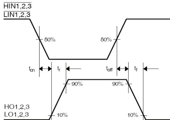
Fig 4. Input/Output Switching Time Waveform Definitions
