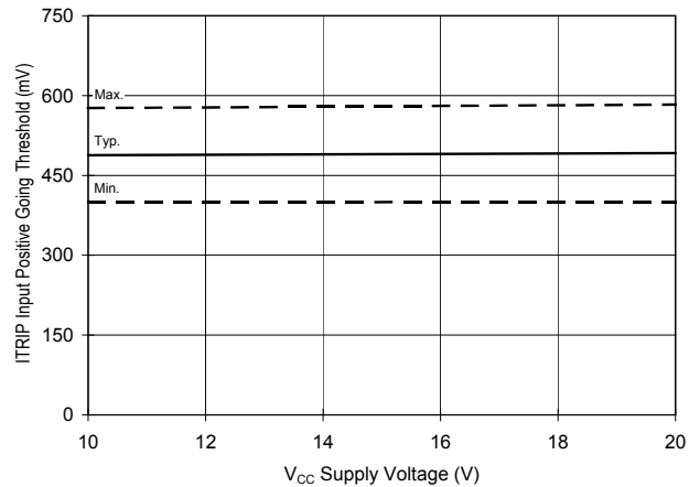
Fig 23b. ITRIP Input Positive Going Threshold
