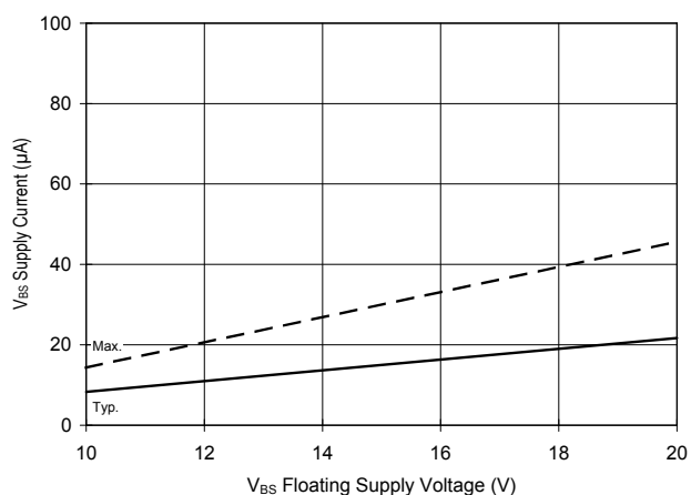
Fig 27b. V BS Supply Current Vs. Voltage
