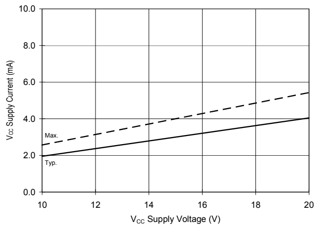
Fig 28b. V CC Supply Current Vs. Voltage
