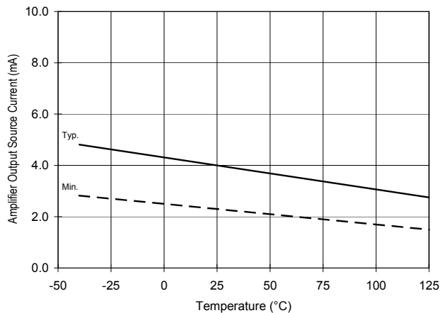
Fig 46a. Amplifier Output Source Current Vs. Temperature
