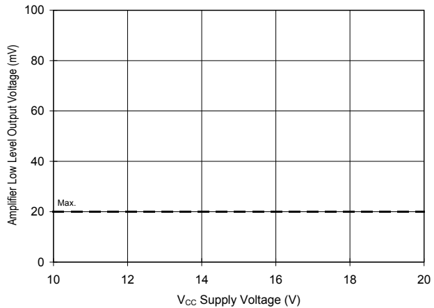
Fig 45b. Amplifier Low Level Output Vs. Voltage
