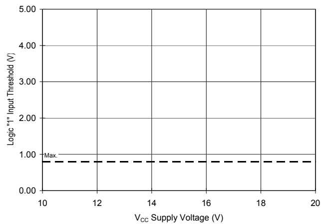
Fig 22b. Logic "1" Input Threshold Vs. Voltage
