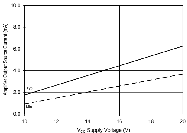
Fig 46b. Amplifier Output Source Current Vs. Voltage
