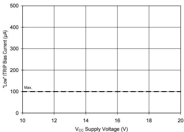
Fig 32b. "Low" ITRIP Current Vs. Voltage
