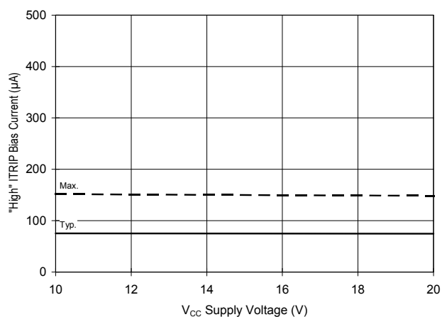
Fig 31b. "High" ITRIP Current Vs. Voltage
