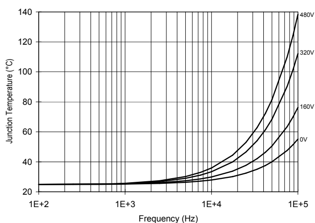
Fig 53. IR2130 T_J Vs. Frequency (IRF450) R_{GATE} = 10\Omega , V_{CC} = 15V
