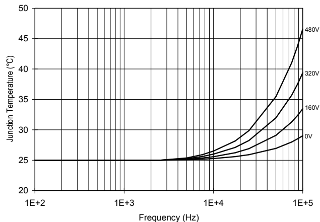
Fig 50. IR2130 T_J Vs. Frequency (IRF820) R_{GATE} = 33\Omega , V_{CC} = 15V
