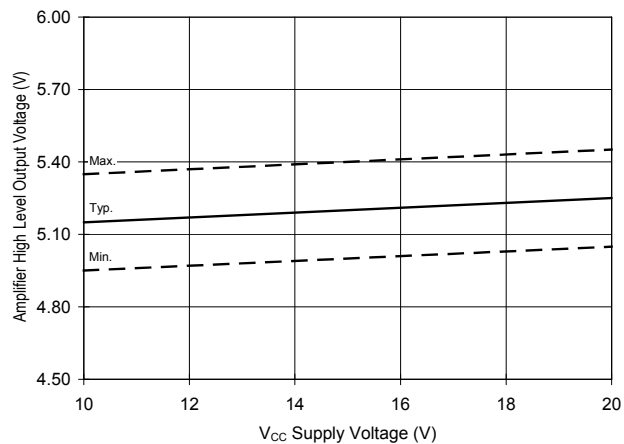
Fig 44b. Amplifier High Level Output Vs. Voltage
