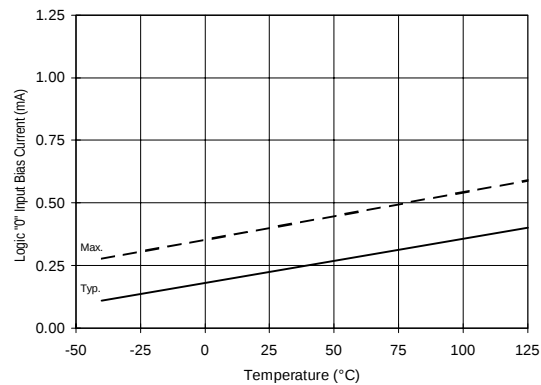
Figure 30A. Logic “0” Input Current vs. Temperature
