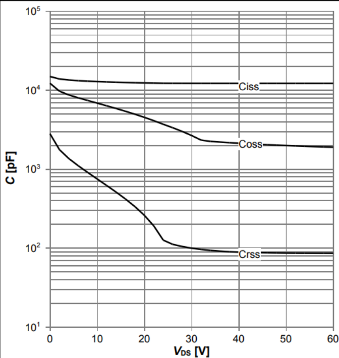
Diagram 11: Typ. capacitances
