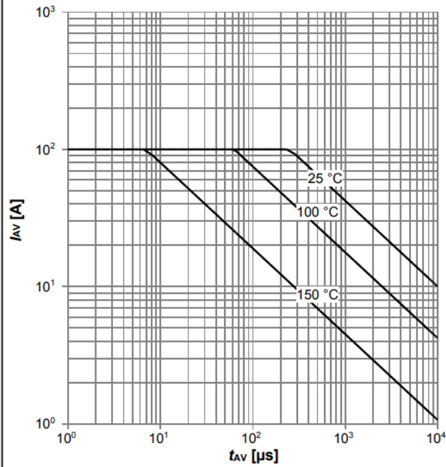
Diagram 13: Avalanche characteristics
