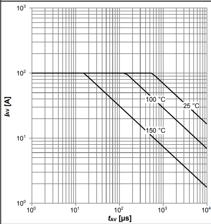
Diagram 13: Avalanche characteristics
