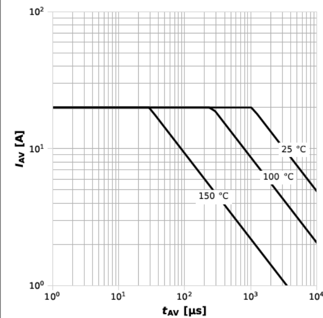
Diagram 13: Avalanche characteristics
