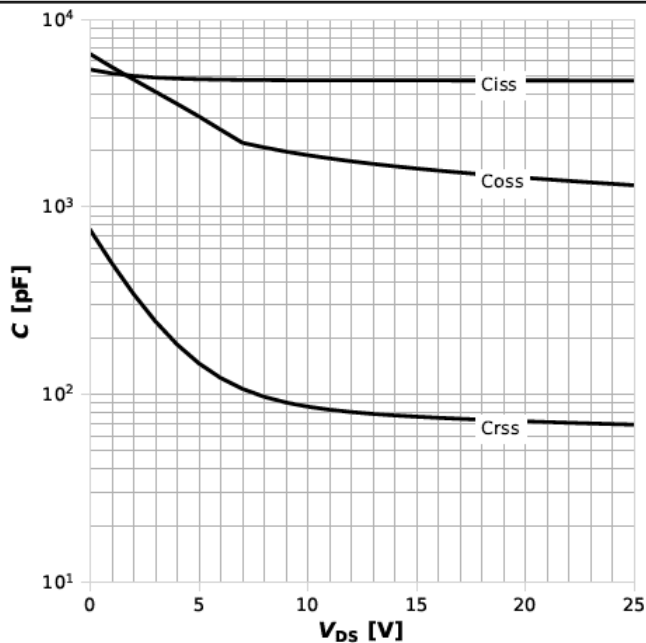
Diagram 11: Typ. capacitances
