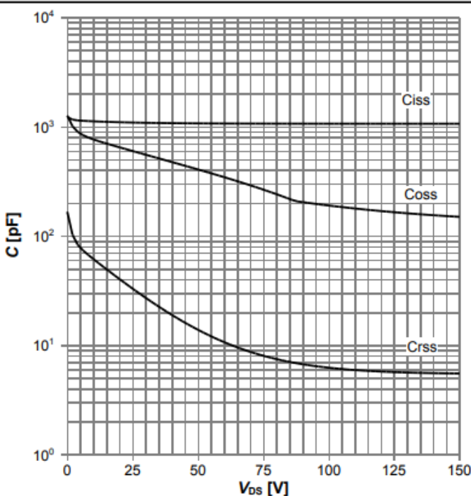
Diagram 11: Typ. capacitances
