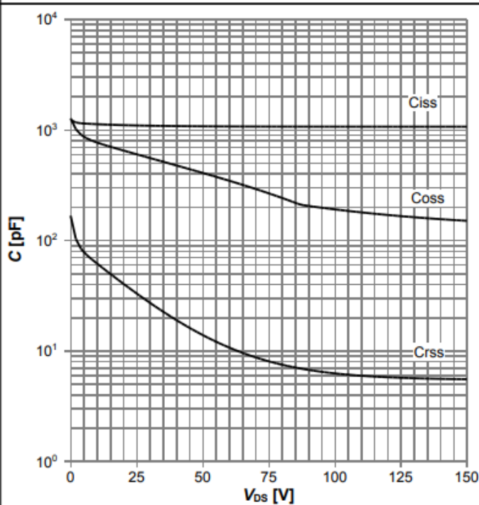
Diagram 11: Typ. capacitances
