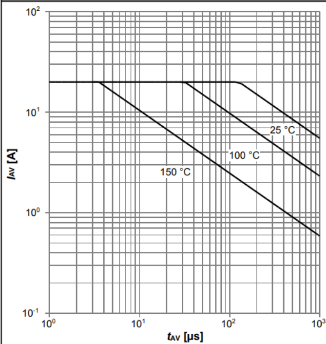
Diagram 13: Avalanche characteristics
