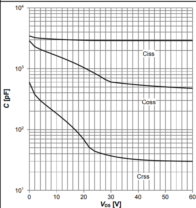
Diagram 11: Typ. capacitances
