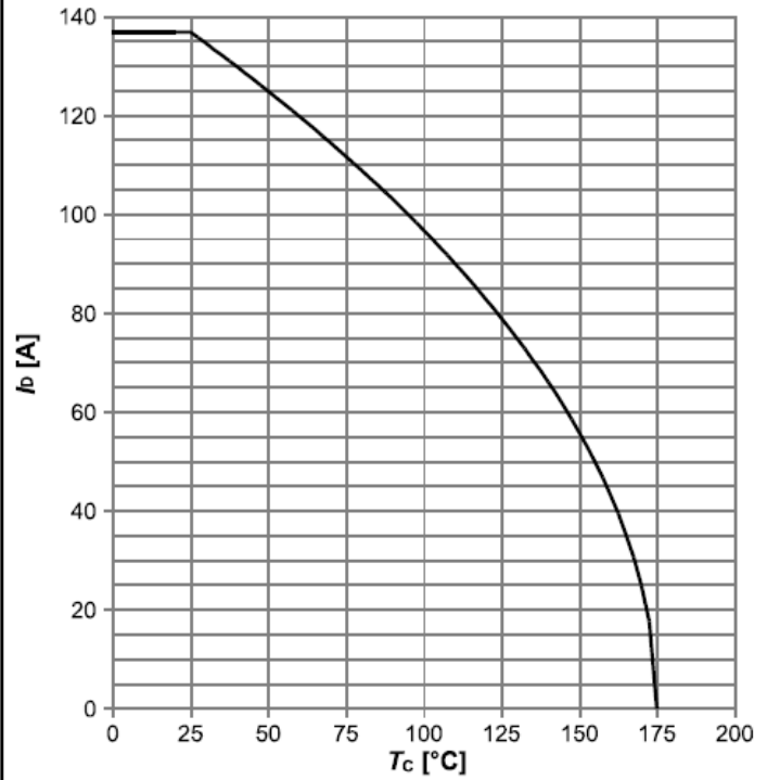
Diagram 2: Drain current
