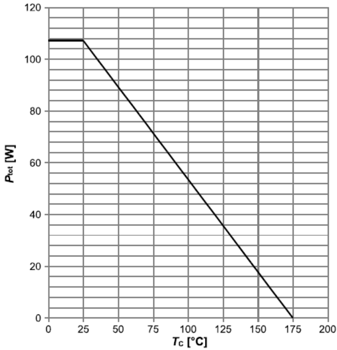
Diagram 1: Power dissipation
