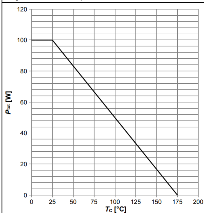
Diagram 1: Power dissipation
