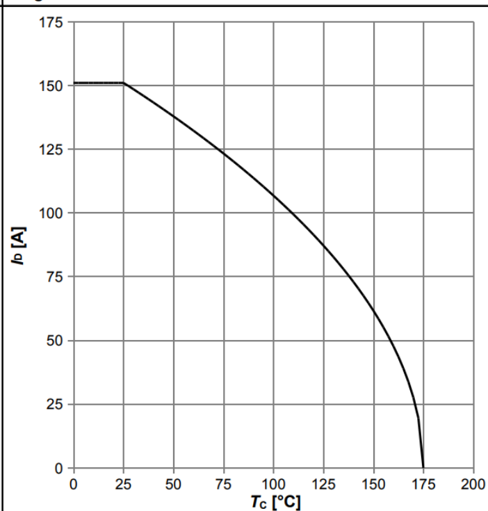
Diagram 2: Drain current
