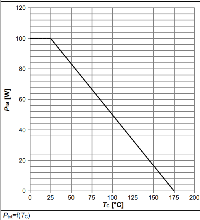
Diagram 1: Power dissipation
