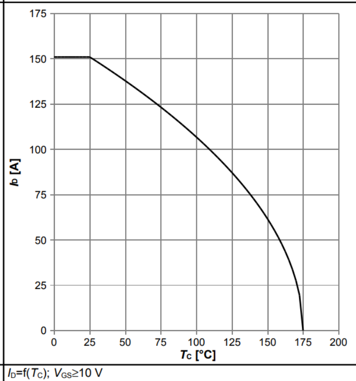
Diagram 2: Drain current
