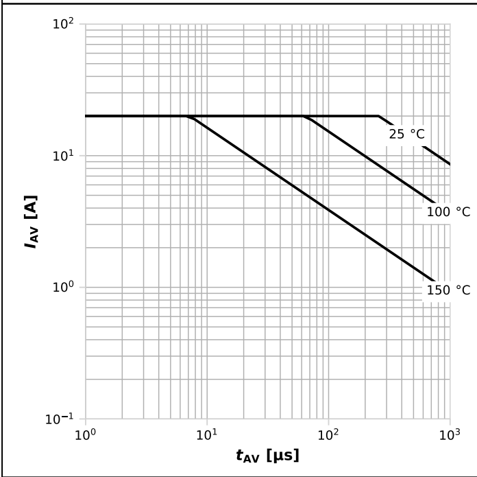
Diagram 13: Avalanche characteristics
