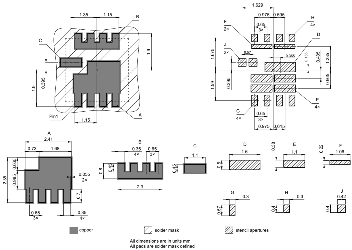
Figure 2 Footprint drawing PG-TTFN-9, dimensions in mm
