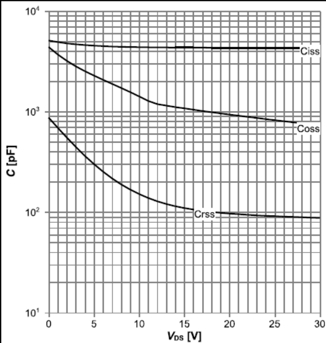
Diagram 11: Typ. capacitances
