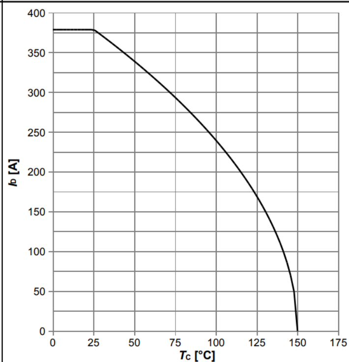
Diagram 2: Drain current
