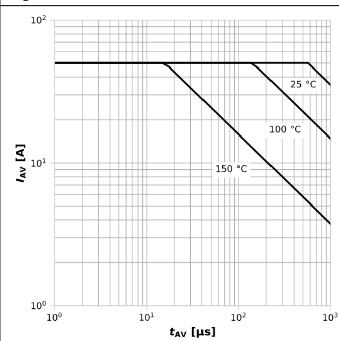
Diagram 13: Avalanche characteristics
