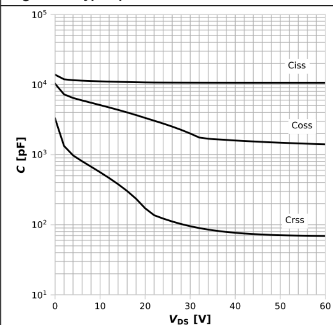
Diagram 11: Typ. capacitances
