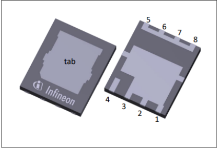
PG-WHSON-8
