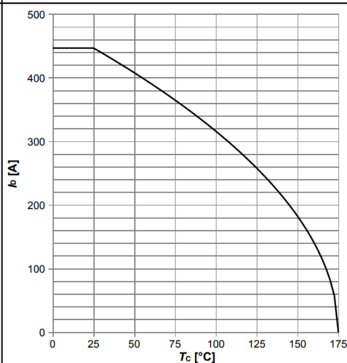
Diagram 2: Drain current
